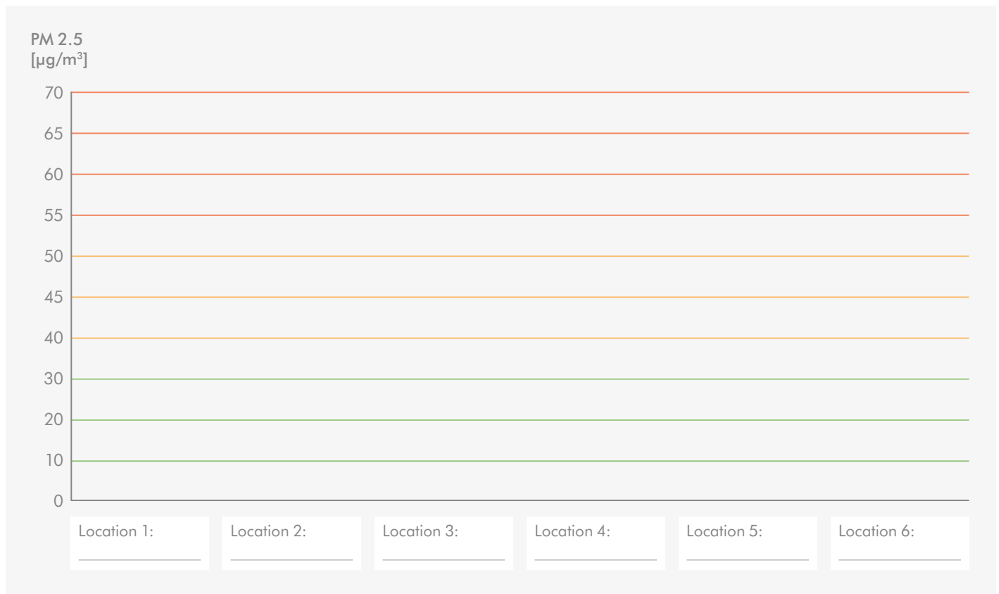
Graph 01 – Particulate pollution
