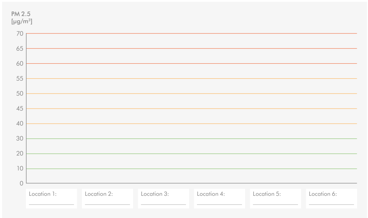
Graph 01 – Particulate pollution (PM2.5)
