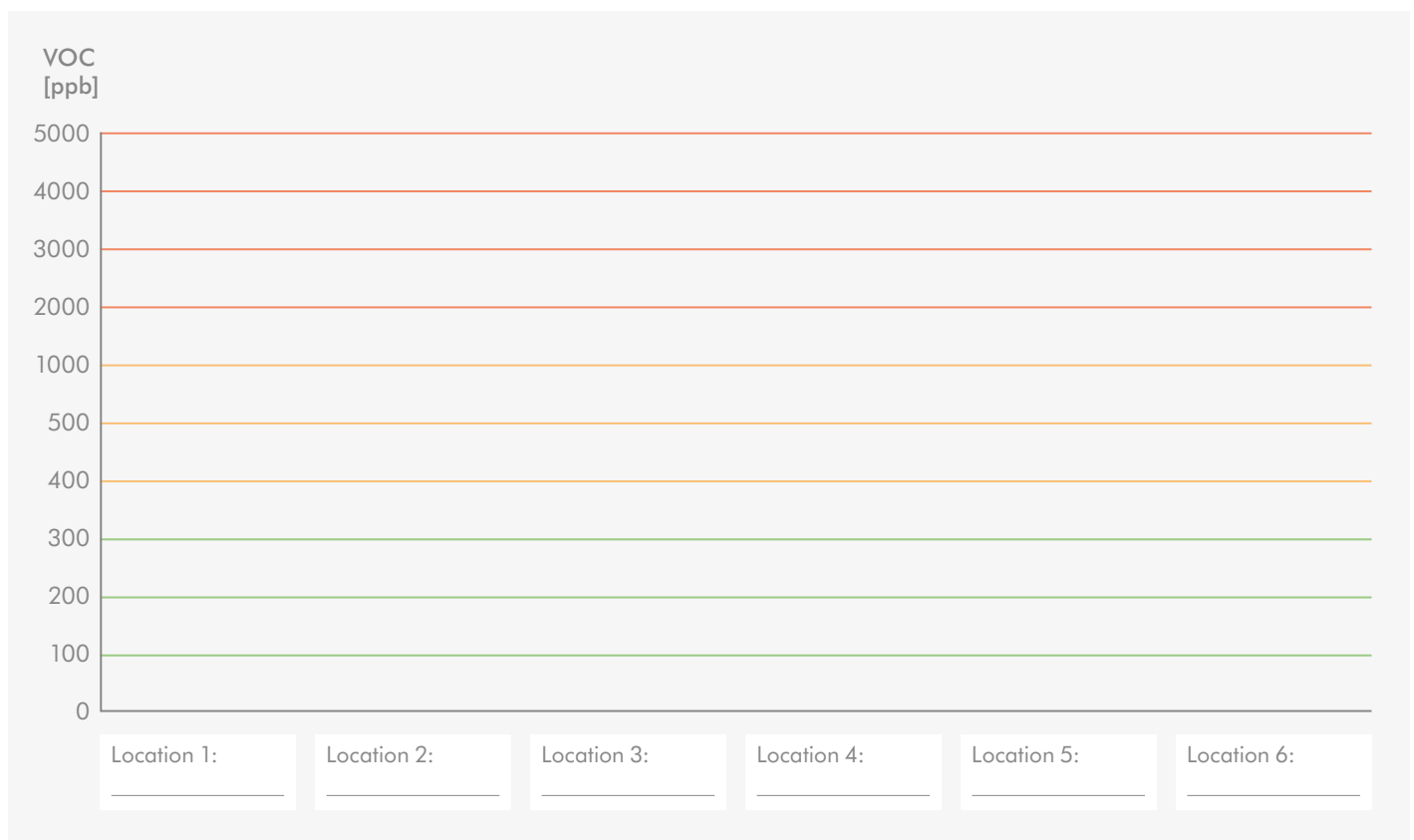
Graph 02 – Gas pollution
