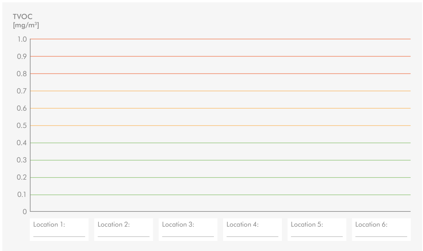
Graph 03 – Gas pollution (TVOC) (mg/m 3 )
